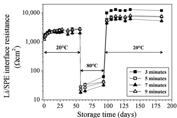
Fig. 7. Time evolution of the interfacial resistance of cross-linked PEO-LiTFSI-PYR 14 TFSI ternary polymer electrolytes in contact with lithium metal electrodes. The electrolyte samples were processed with different UV photo-irradiation times (see legend). The interfacial resistance is normalized with respect to the lithium electrode active area.
